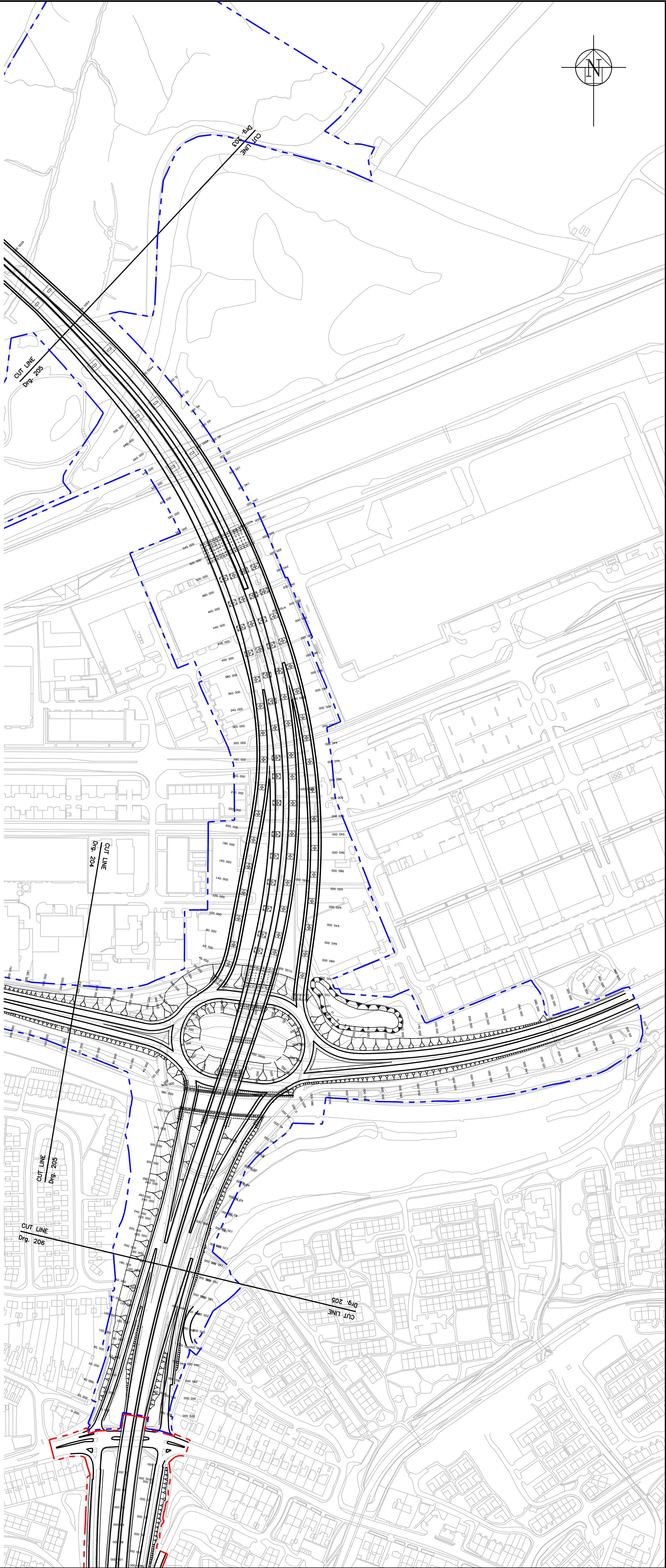
PLAN
